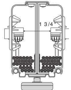
AO2 Non-Powered Panel Wiring Schematic
